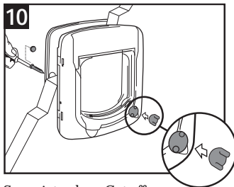
Screw into place. Cut off excess screw with wire cutters. Cover screw holes with blanking plugs for neat finish. Push fit 4-way locking handle into place.
